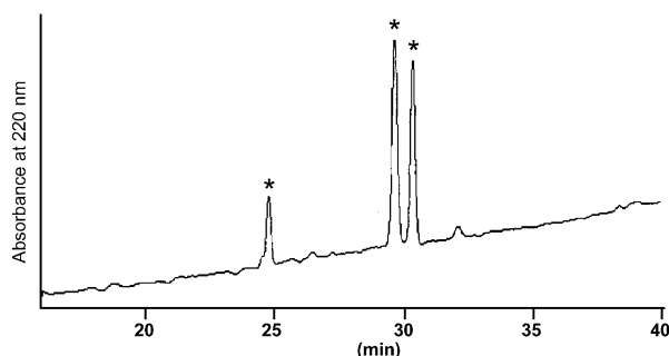
Figure 3. HPLC analysis of biotinylated analogue ( 13 ), which was eluted using a linear gradient of 20–80% acetonitrile containing 0.1% TFA in 60 min. Peaks were detected at 220 nm. Three peaks corresponding to each isomers of 13 are marked with an asterisk.
