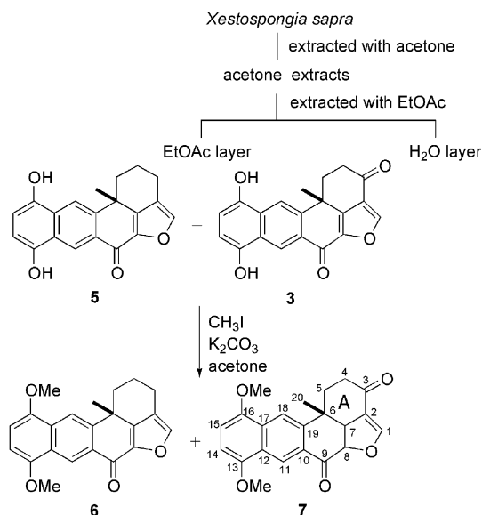
Scheme 1. Preparation of marine sponge extract, and derivatization of hydroquinone components to dimethyl ethers.
