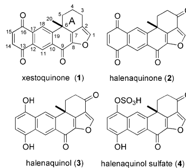
Figure 1. Xestoquinone and its analogues.
