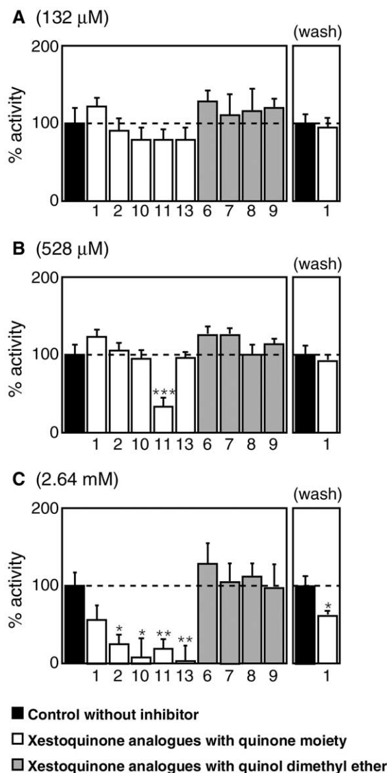
Figure 2. Effects of xestoquinone ( 1 ) and its analogues on myosin Ca 2+ ATPase activity: (A) test at substance concentration of 132 μM; (B) test at substance concentration of 528 μM; (C) test at substance concentration of 2.64 mM. 'Wash' indicates that the well was washed with the assay buffer after incubation. The ordinate gives the relative phosphoric acid value; the phosphoric acid value corresponding to lack of inhibitor was designated as 100% (dashed line). Values are given as means ± SE ( n = 4). Values significantly different from the control value (without inhibitor, filled bar) are indicated by asterisks (Student's t -test, * p < 0.05, ** p < 0.01, *** p < 0.005).
