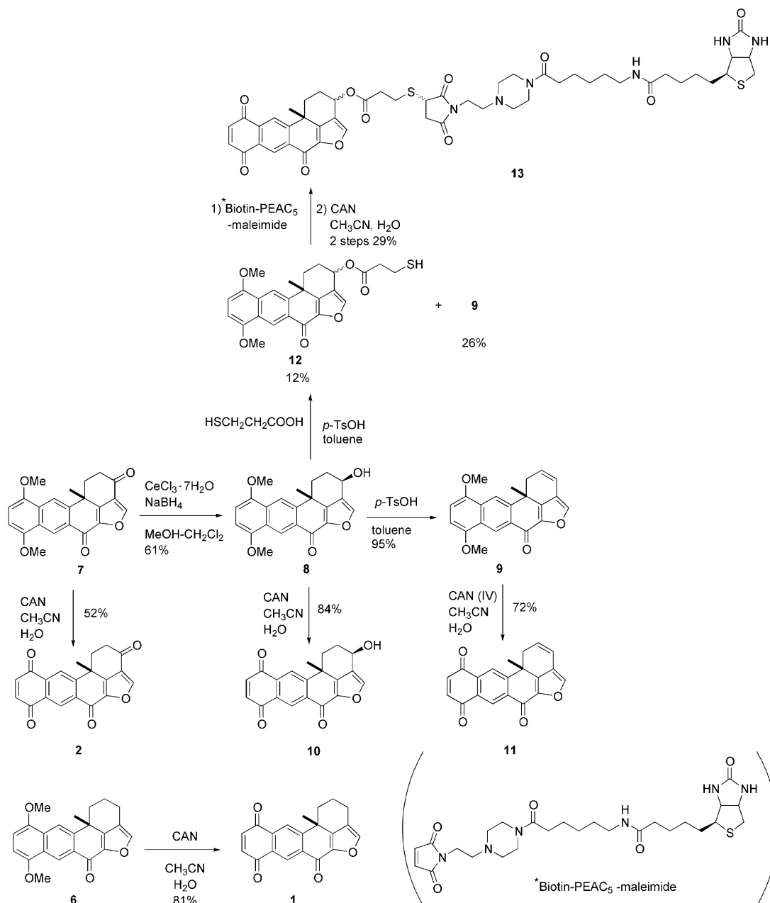
Scheme 2. Derivatization of various xestoquinone analogues.
